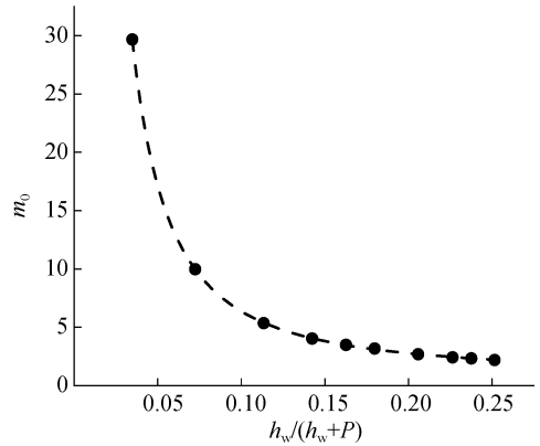
图9 堰槽组合流量系数随相对作用水头的变化 Fig. 9 Change of flow coefficient of weir and flume combination
